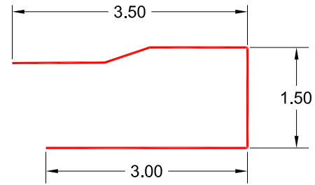
MIRAMESH® TR - TYPICAL DIMENSION DETAIL
