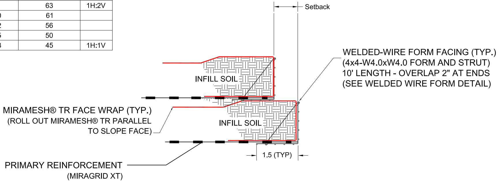
MIRAMESH® TR - TYPICAL DIMENSION DETAIL
