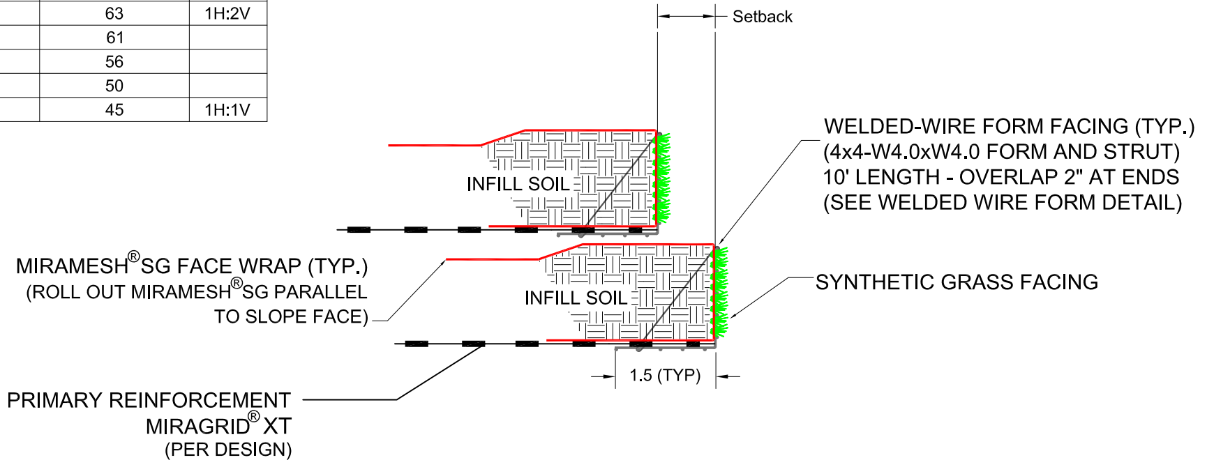
MIRAMESH® SG - TYPICAL DIMENSION DETAIL
