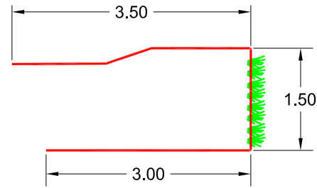
MIRAMESH® SG - TYPICAL DIMENSION DETAIL
