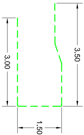
MIRAMESH®GR - TYPICAL DIMENSION DETAIL
