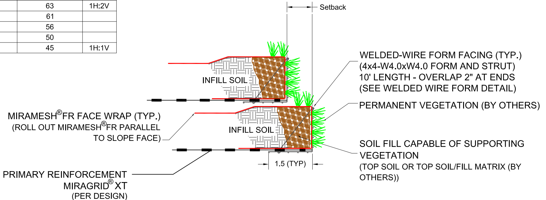
MIRAMESH® FR - TYPICAL DIMENSION DETAIL
