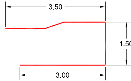
MIRAMESH® FR - TYPICAL DIMENSION DETAIL
