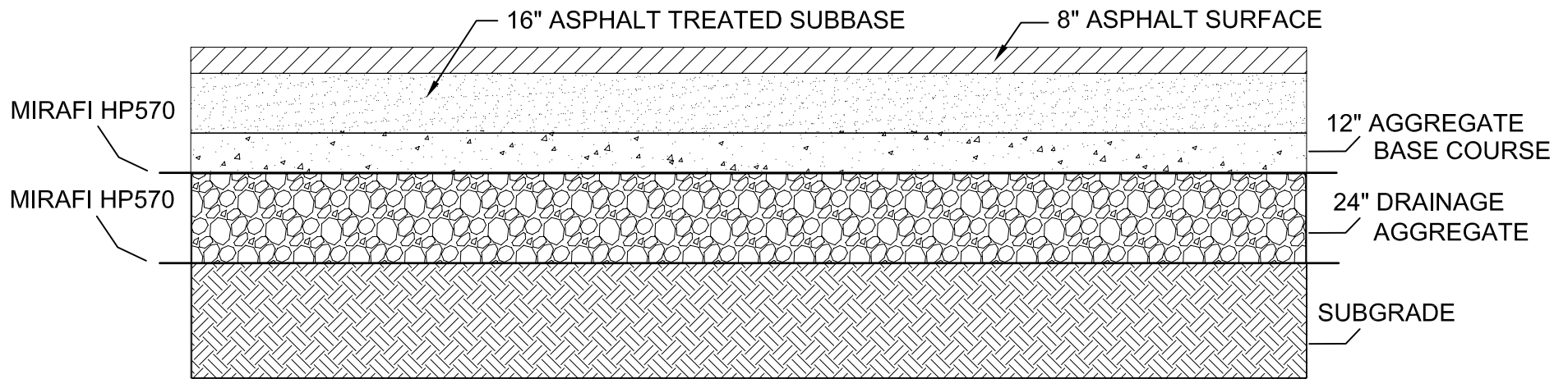
DETAIL FOR SUBGRADE STABILIZATION NOT TO SCALE
