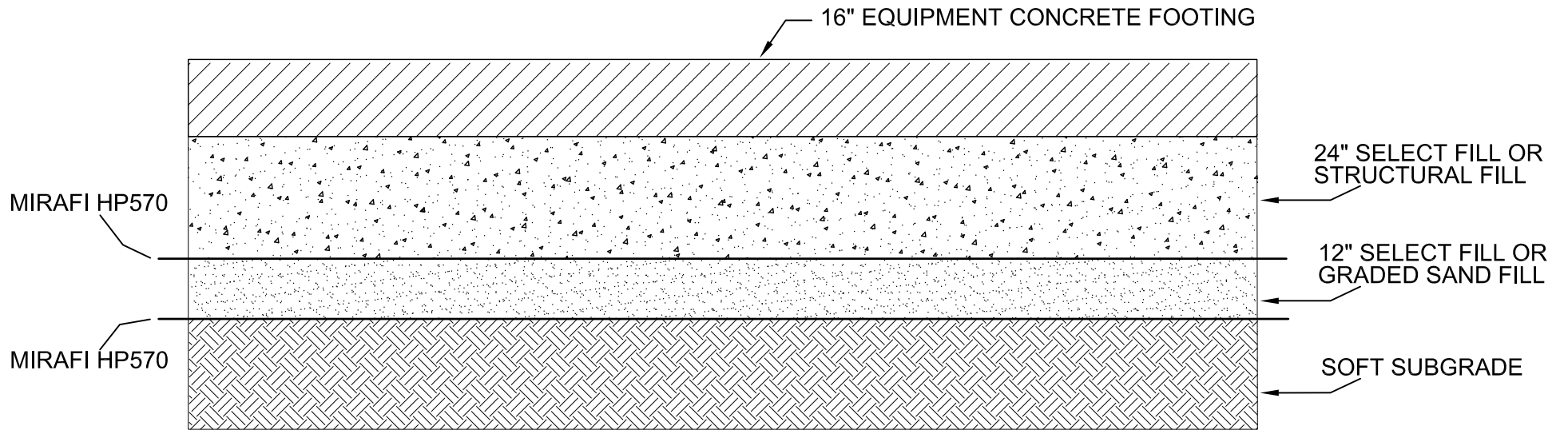
DETAIL FOR SUBGRADE STABILIZATION NOT TO SCALE
