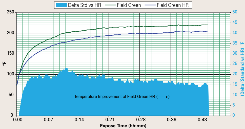
Temperature build-up vs exposure time in Field Green Color Standard vs Field Green HR Formula. HR formulation improvement vs Control at exposure temperature greater than 140°F Average Improvement...17.5 °F Minimum Improvement...14.0 °F Maximum Improvement...23.0 °F Sigma...1.8 °F
